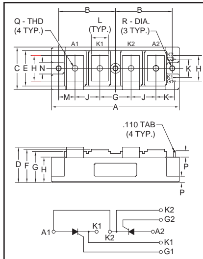
Outline Drawing
