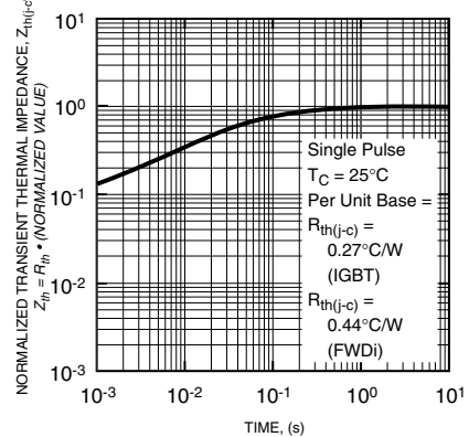
TRANSIENT THERMAL IMPEDANCE CHARACTERISTICS (IGBT & FWD) - BRAKE PART
