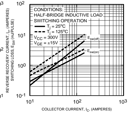
SWITCHING LOSS CHARACTERISTICS
