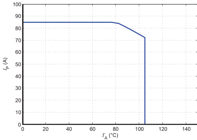
Figure 23: I_p vs T_A for LESR 25-NP
