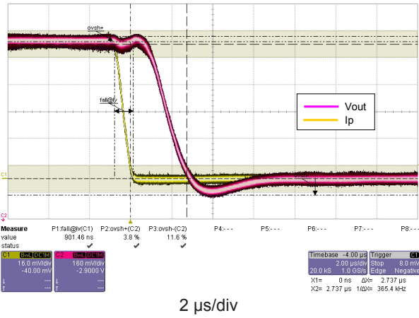
Figure 3: Step response
