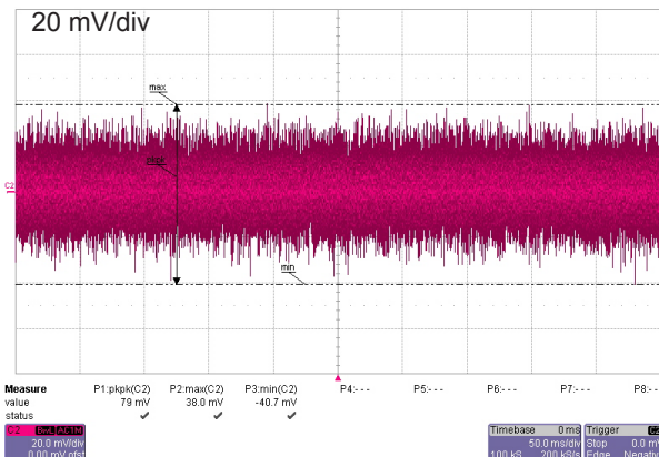
Figure 5: Output noise
