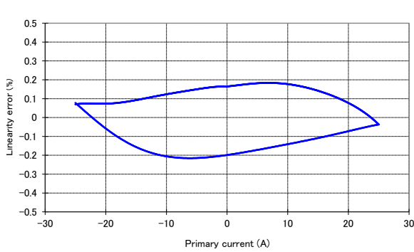
Figure 11: Linearity error
