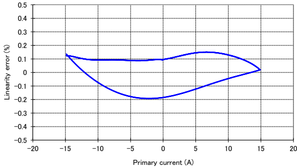
Figure 6: Linearity error
