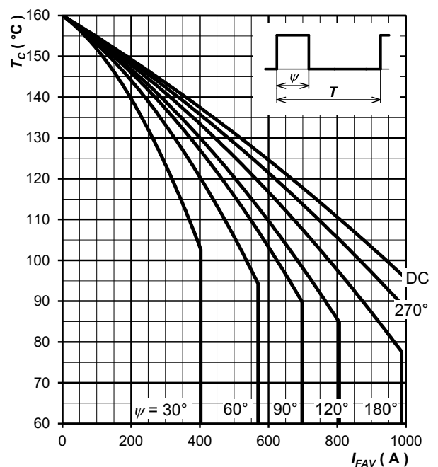
Fig. 8 Max. case temperature vs. aver. forward current, square waveform, f = 50 Hz, T = 1/f
